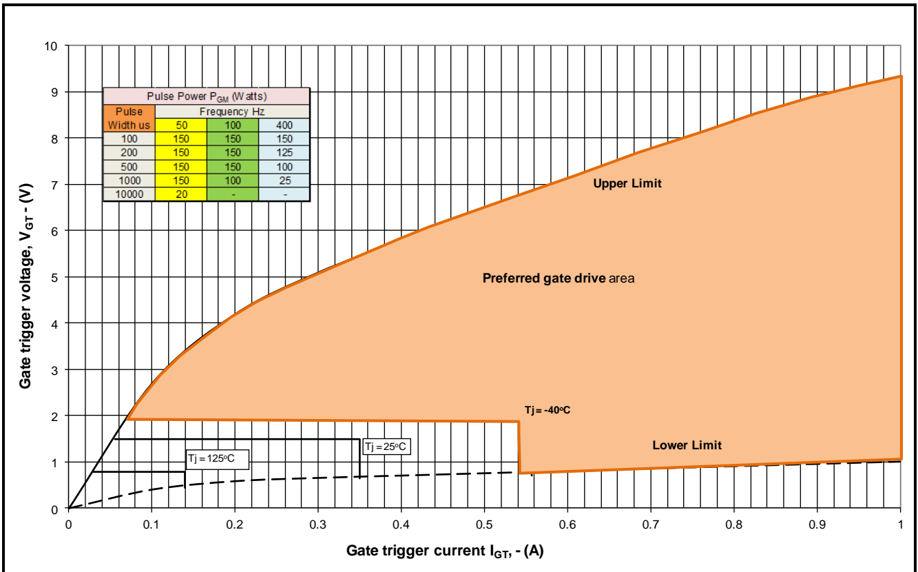
Fig14 Gate Characteristics
